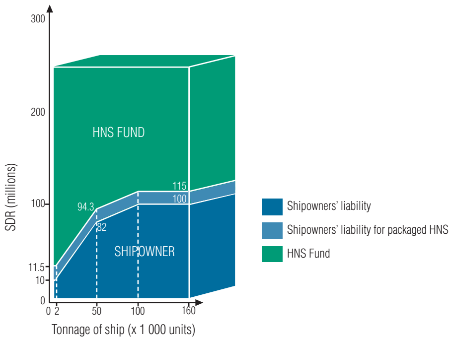
Figure 1. Compensation amounts under the 2010 HNS Convention
